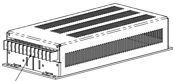
CURTIS 3800 SERIES 12 POLE SINGLE ROW BARRIER TYPE TERMINAL WITH 6-32 UNC SCREWS
