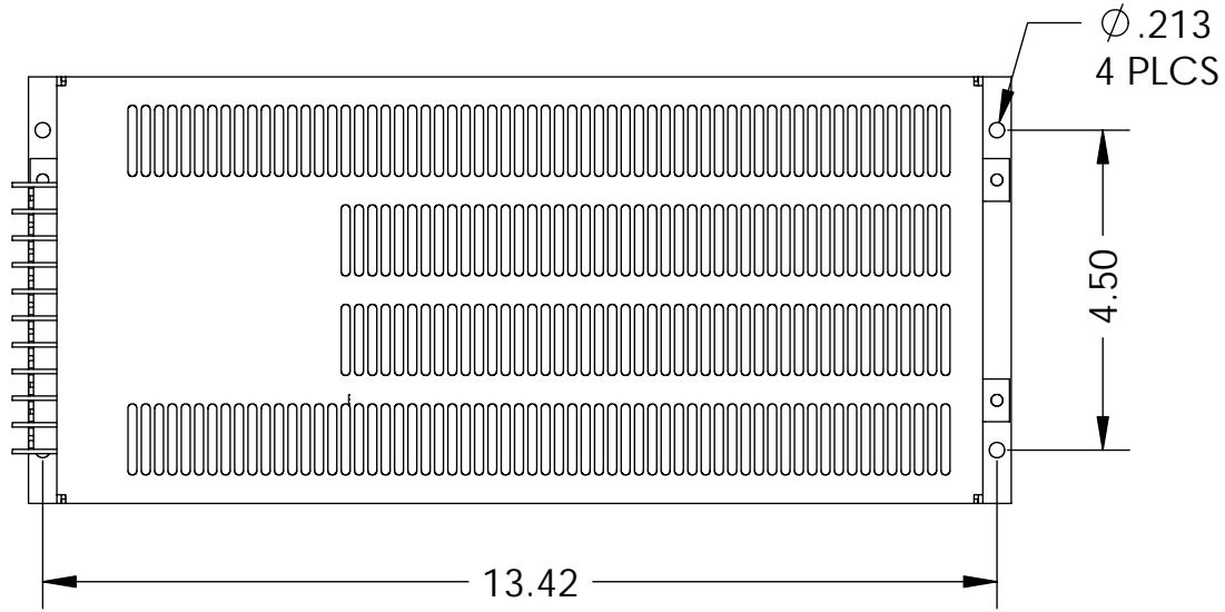
CURTIS 38000 SERIES SINGLE ROW BARRIER TYPE TERMINAL WITH #6 SCREWS
