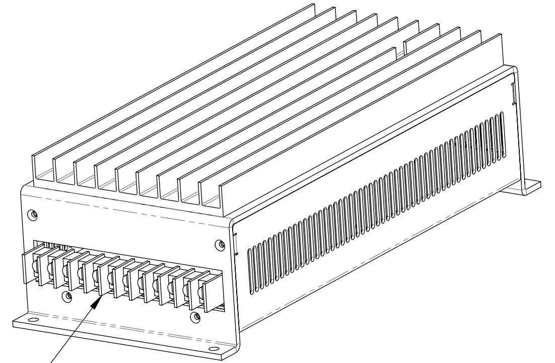
12 Pole barrier type of terminal with M3.5 screws
